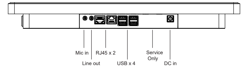
15.6" Ultron Windows Touchscreen ULT156 PART#1215U ULT156 PART#1235U
